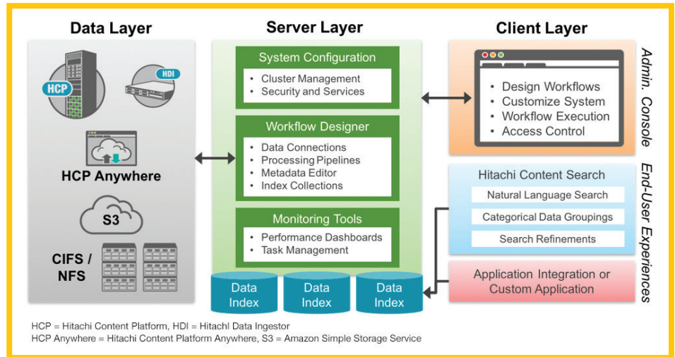
Figure 1. Hitachi Content Intelligence Architecture
