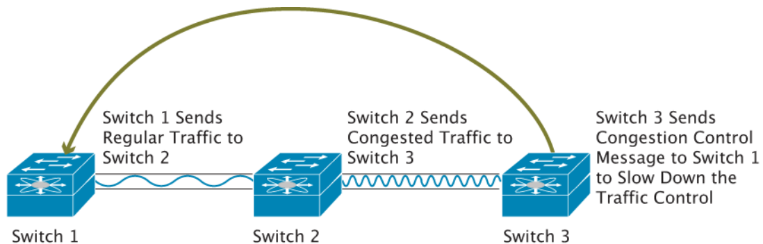
Figure 7. FCC Congestion Mitigation and Blocking
