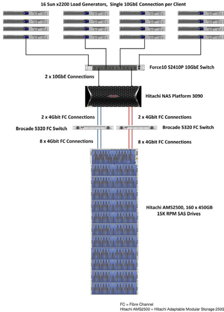
Figure 2. High-level Configuration Overview
